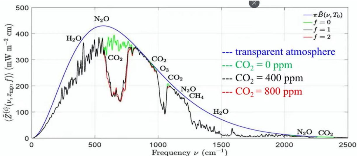
Figure 2: The IR spectrum of the earth with a transparent atmosphere, with fixed amounts of \text{H}_2\text{O} , \text{N}_2\text{O} , \text{CH}_4 , and \text{O}_3 , and with 0 ppmv, 400 ppmv, and 800 ppmv of \text{CO}_2 . [1, graph from 2] The smooth upper line represents the IR emitted by the surface, the so-called blackbody curve.
