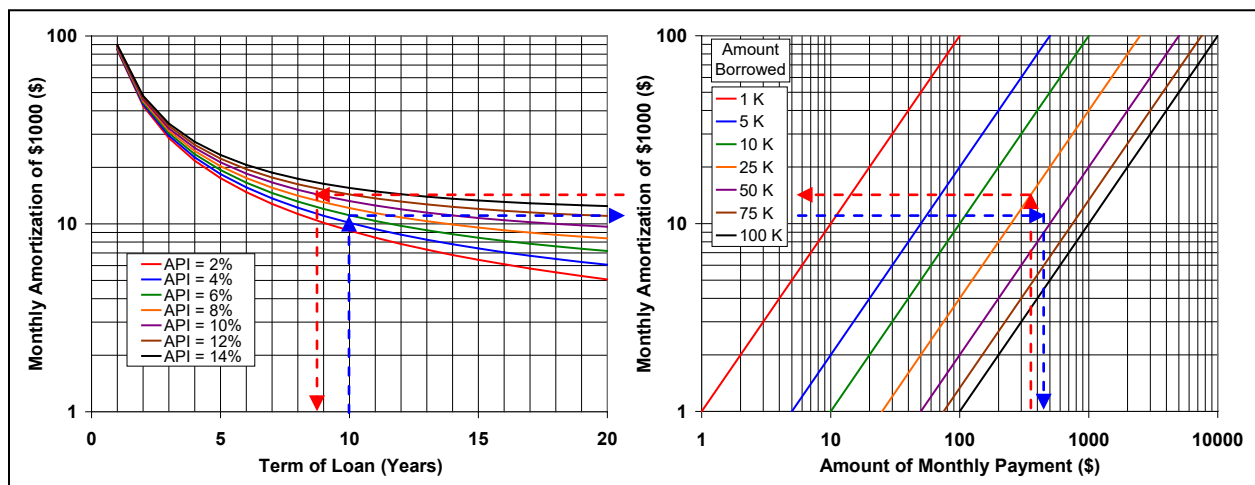
Figure 5-2: Nomogram for Student Loan Repayment
