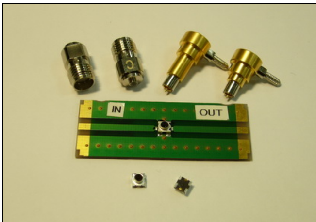
As shown: Sunridge SWD-TP & SWD-TPL test probe and SWDTP-SMAJ Adapter
